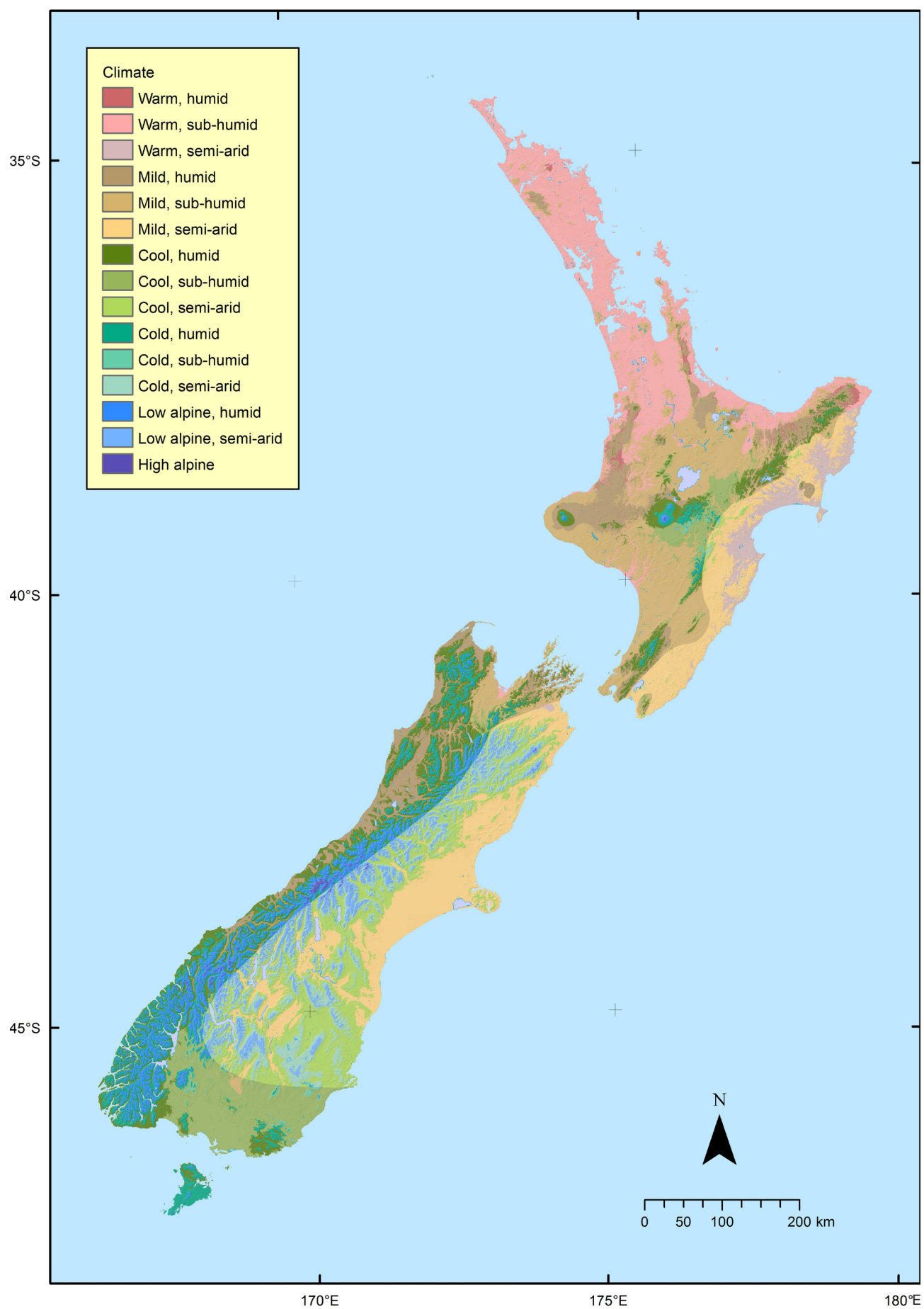
Figure 1. Macroclimatic zones of New Zealand.
