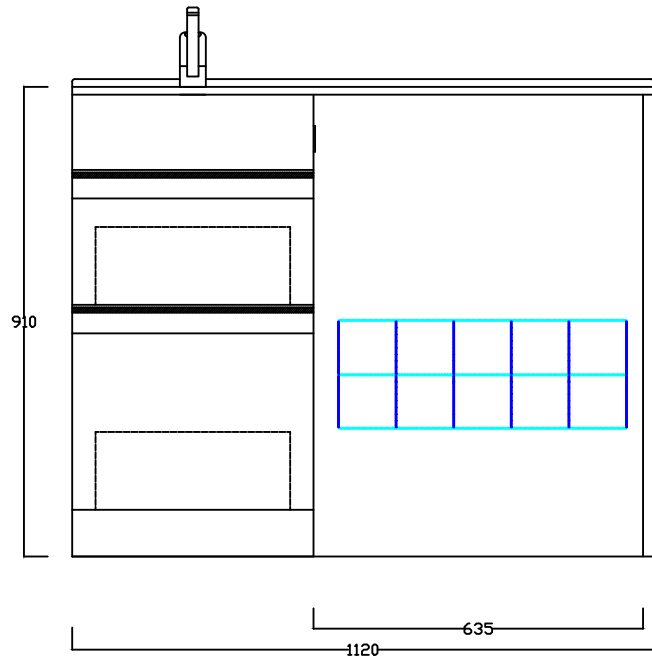
Front Loader Laundry Center FL1120 for Right hand tub version mirror views. 27/10/2018
