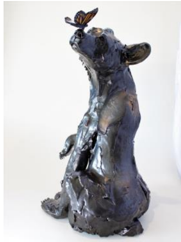
Balancing Act
